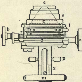
Fig. 51a. Complete Substage. Front view.
