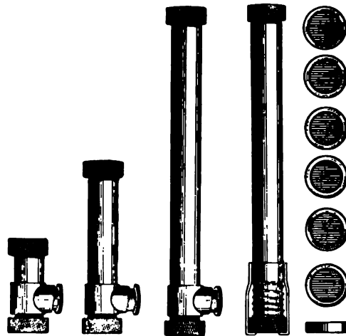
FIG. 46.—U. S. Geological Survey Apparatus for Measuring the Color of Water.
