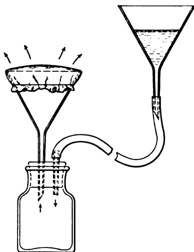
FIG. 7.—Apparatus for Concentrating Microscopic Organisms.
