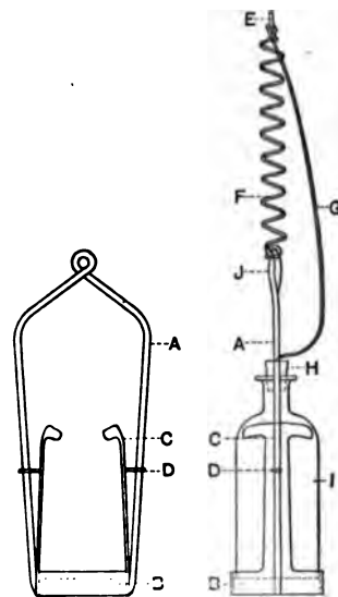
FIG. 1.—Apparatus for Collecting Samples of Water. After Whipple.
