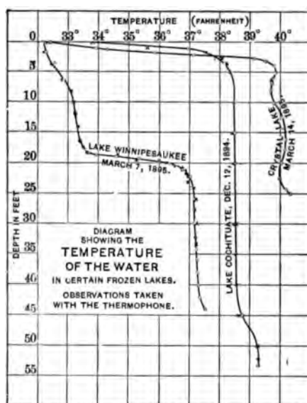
FIG. 38.—Temperature of Water in Frozen Lakes. After FitzGerald.
