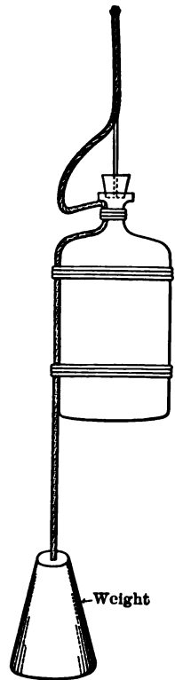
FIG. 2.—Rig for Binding Bottle to Rope and for Drawing the Stopper.
