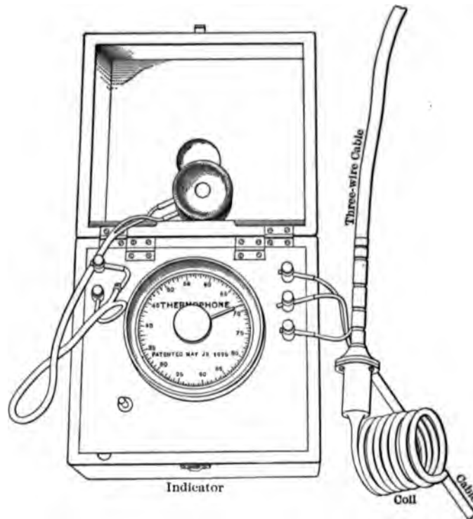
FIG. 36.—Thermophone.
