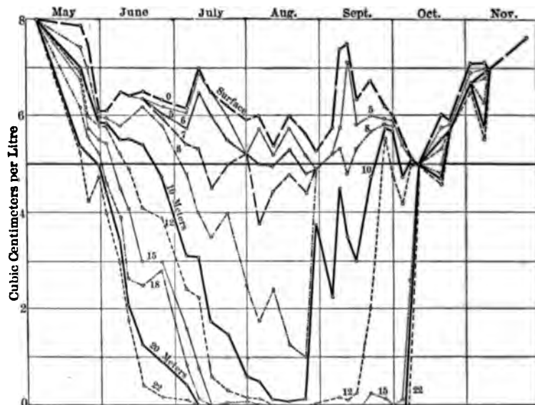
FIG. 50.—Dissolved Oxygen at Different Depths in Lake Mendota. After Birge and Juday.
