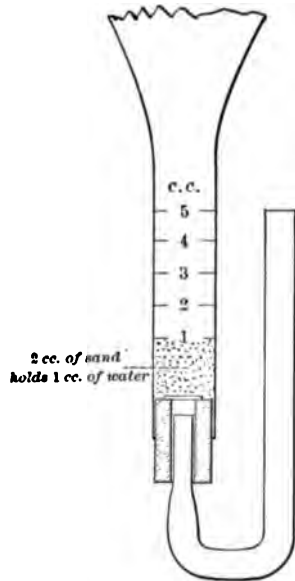
FIG. 15.—Concentrating Attachment.
