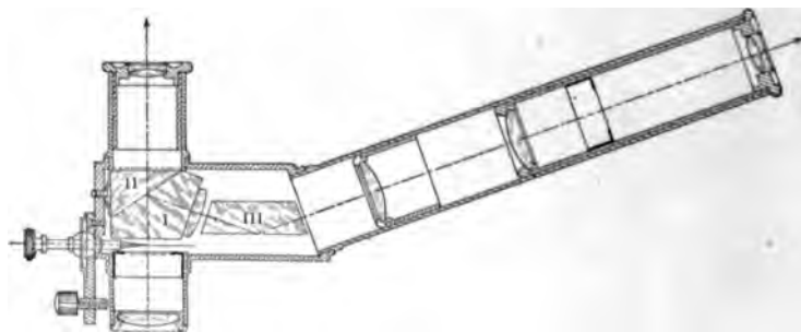
FIG. 31.—Leitz Double Demonstration Eye-piece.
