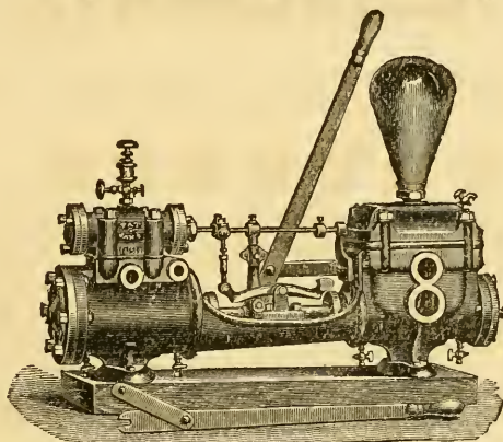
Cut above represents regular Boiler Feed Pump, Nos. 3 and 4. Showing New Patent Valve Motion, and Hand Power LEVER Attached and Detached.
