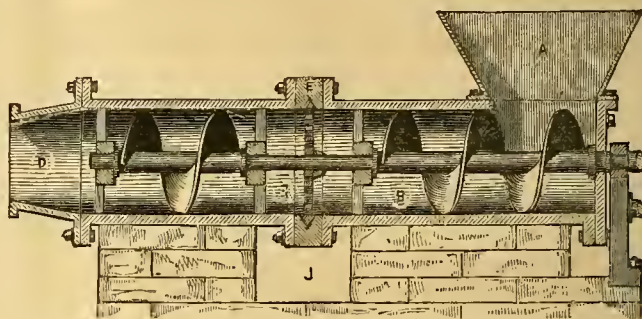
Fig. 1.—Side View of Brick Machine.
