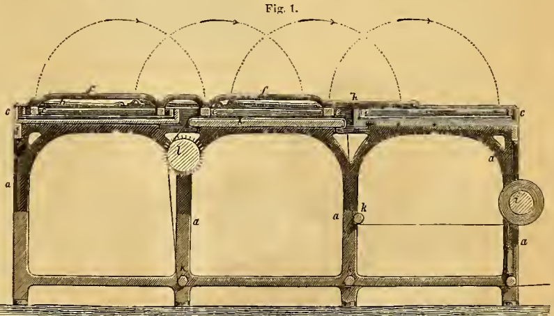
Fig. 1 of our engravings is a longitudinal section of the apparatus, as contrived for printing with two blocks. Fig. 2 is a plan cor-
